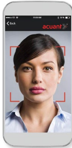
Facial Recognition
