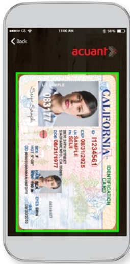
Capture & Classify
