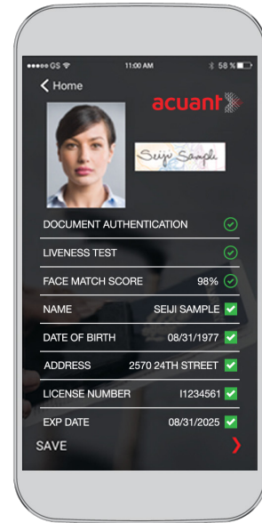
AUTHENTICATION
