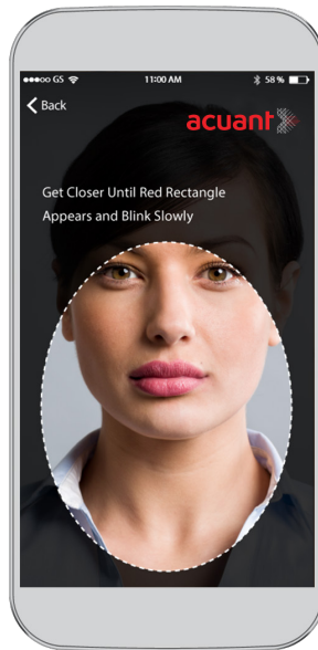
FACIAL RECOGNITION
