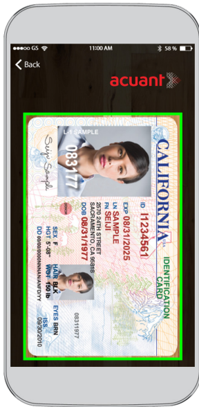
CAPTURE & CLASSIFY
